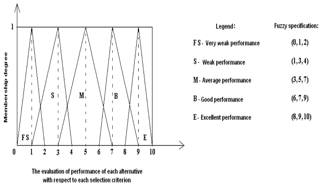
Figure 5 - Fuzzy evaluations regarding the performance of suppliers with respect to each selection criterion (the picture is from own source)
