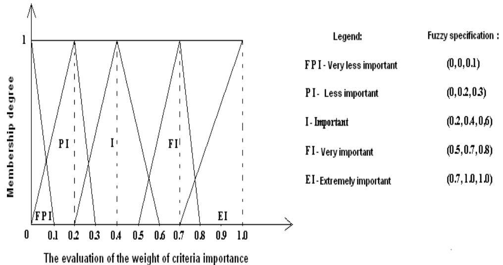
Figure 3 – Fuzzy evaluations regarding the importance weight of criteria (the picture is from own source)
